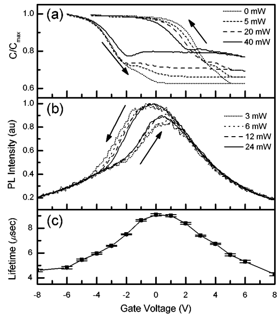
FIG. 2. Capacitance ( C-V ) and photoluminescence (PL) hysteresis loops (a),(b) measured at the same voltage sweep rate (50 mV/s) demonstrate data retention in this device. PL quenching is attributed to nonradiative Auger recombination in charged nanocrystals. PL decay lifetimes recorded at various gate biases (c) suggest that uncharged nanocrystals are also indirectly quenched by exciton migration to charged nanocrystals.
